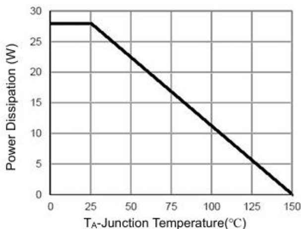
Figure 9 Power De-rating
