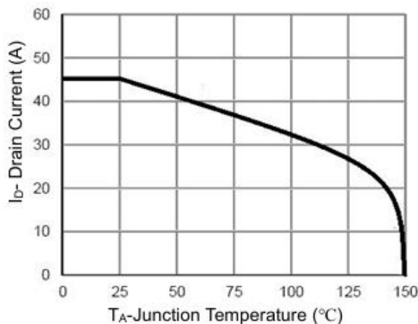
Figure 10 Current De-rating
